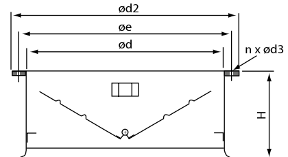
VKVE/F
